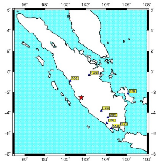
Figure 1. Epicenter of the Mainshock, 01-10-2009 Event (Red Star), Stations Distribution (Blue Triangles)
